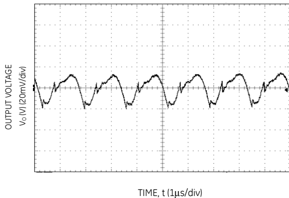
Figure 27. Typical output ripple and noise (Co=10µF ceramic, VIN = 12V, Io = Io,max.).
