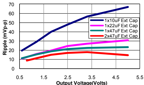
Figure 38. Output ripple voltage for various output voltages with external 1x10µF, 1x22µF, 1x47µF and 2x47µF ceramic capacitors at the output (3A load). Input voltage is 12V.
