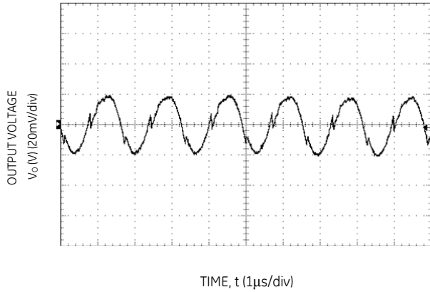
Figure 33. Typical output ripple and noise (Co=10µF ceramic, VIN = 12V, Io = Io,max.).
