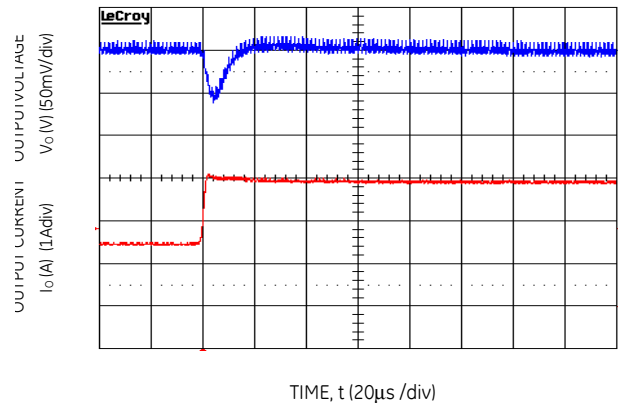
Figure 28. Transient Response to Dynamic Load Change from 50% to 100% at 12Vin, Cout-2x47uF, CTune-2200pF & RTune-261
