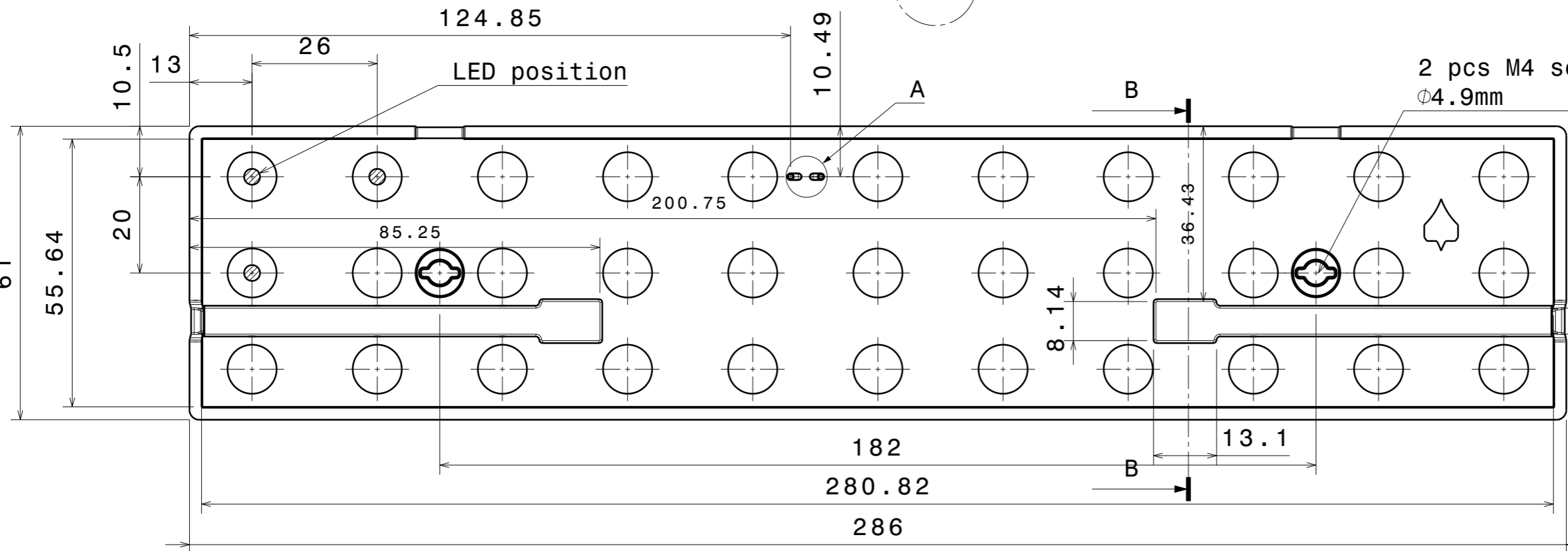
Bottom view
