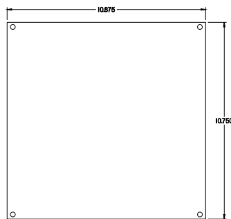
INNER PANEL
