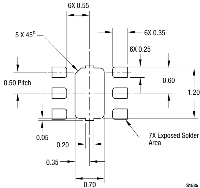
Figure 11. SKY13348-374LF PCB Layout Footprint (Top View)
