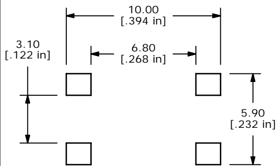
P.C.B MOUNTING
