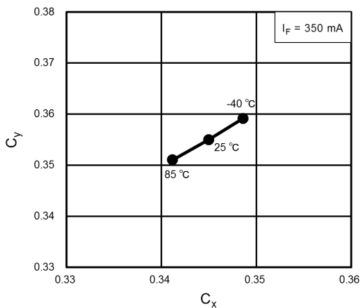
Fig. 8.5 Chromaticity - I_F
