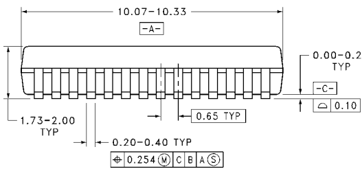
28-Lead Shrink Small Outline Package (SSOP), EIAJ TYPE II, 5.3mm Wide Package Number MSA28
