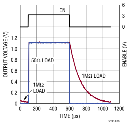
Figure 6. Output Voltage Turn-Off Transient for 1\text{M}\Omega||11\text{pF} and 50\Omega Load Impedance. Input Power 0\text{dBm} , Input Frequency 2140\text{MHz} .
