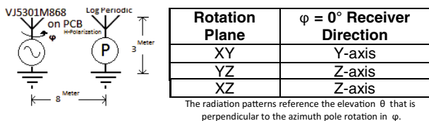
Fig. 3 - VJ5301M868 PCB Mounting and Coordinate Directions
