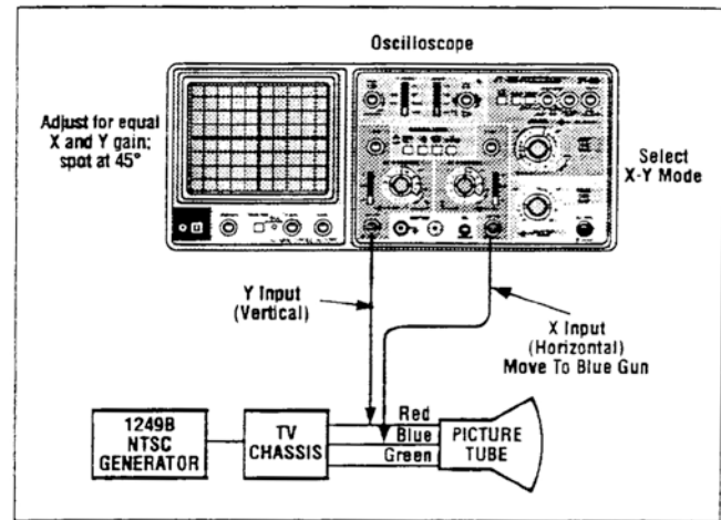
Fig. 6. Using a Conventional Oscilloscope as a Vectorscope, step 2 (set-up).
