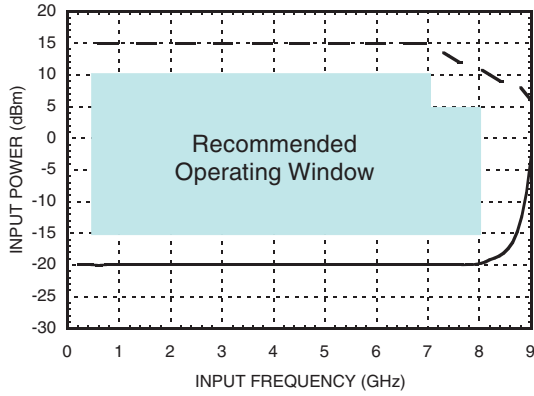
Input Sensitivity Window, T= 25 °C
