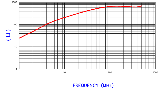
Z vs. FREQUENCY (REF. ONLY)
